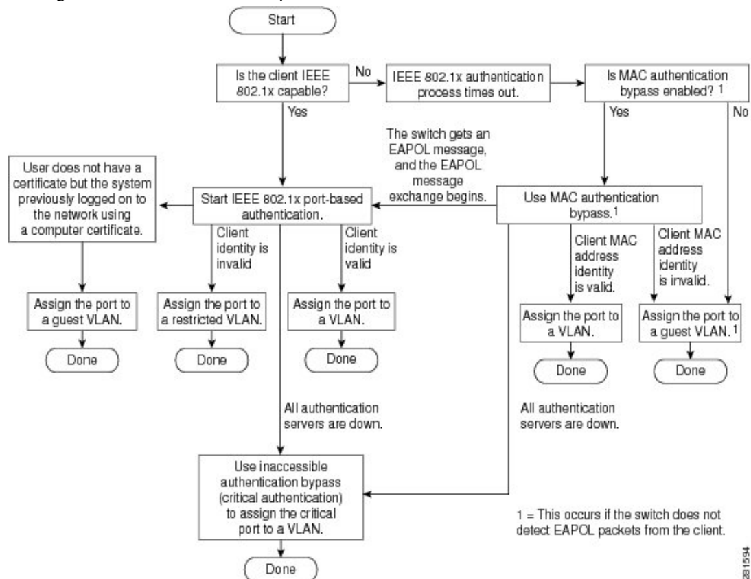
Figure 23: Authentication Flowchart
