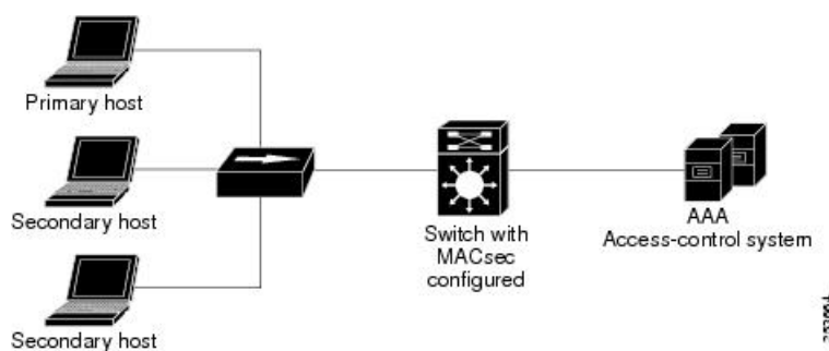
Figure 13: MACsec in Multiple-Host Mode - Unsecured
