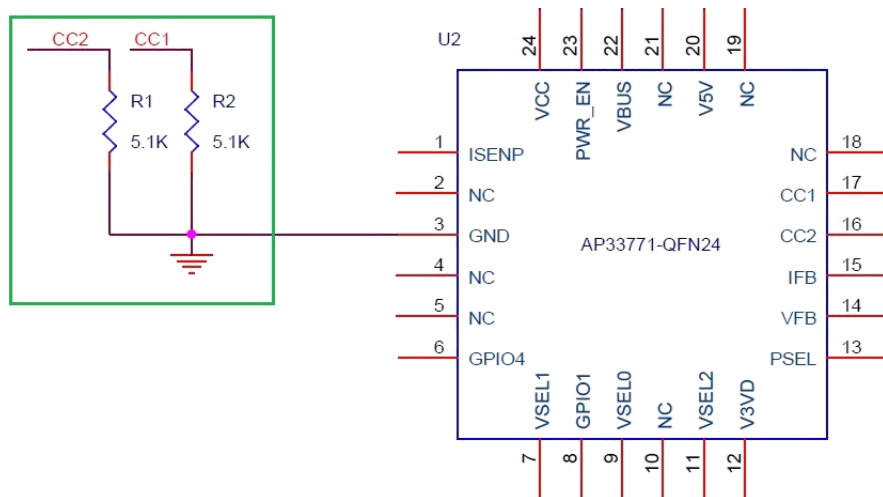
Figure 10 – Make sure the connection of external R_d resistors on CC1 and CC2
