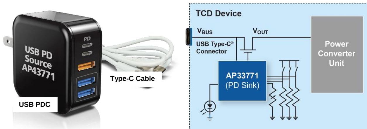
Figure 8 – Examples Based on a Typical TCD Application Scenario with an USB PDC
