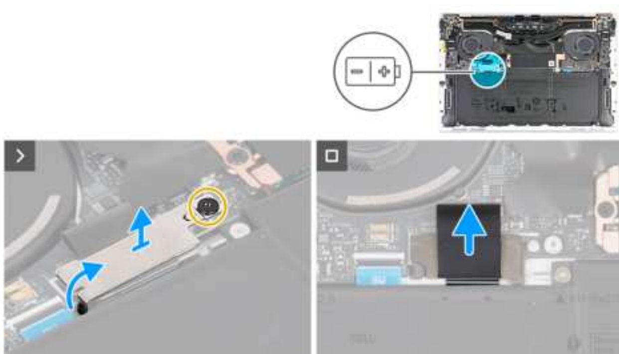
Figure 13. Removing the base cover
