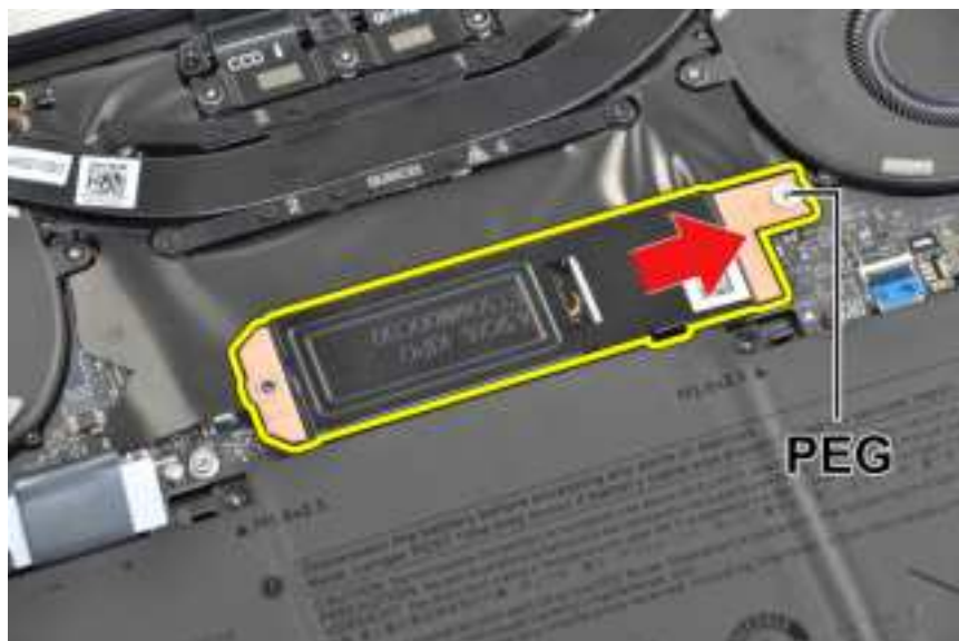
Figure 35. Insert M.2 solid state drive shield
