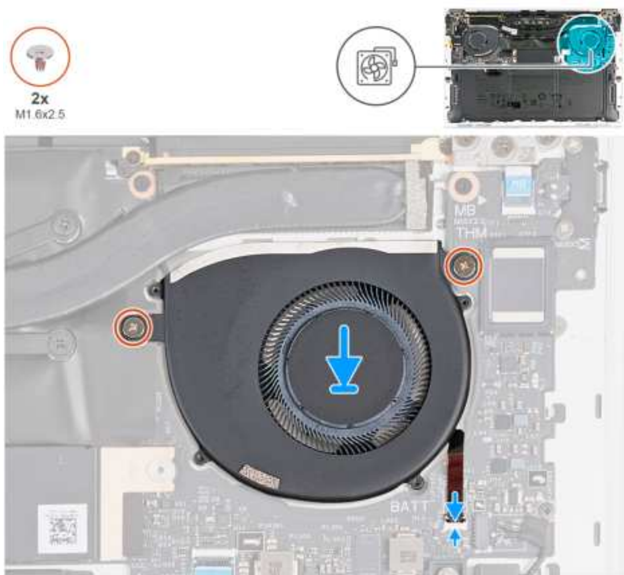
Figure 38. Installing the left/processor fan
