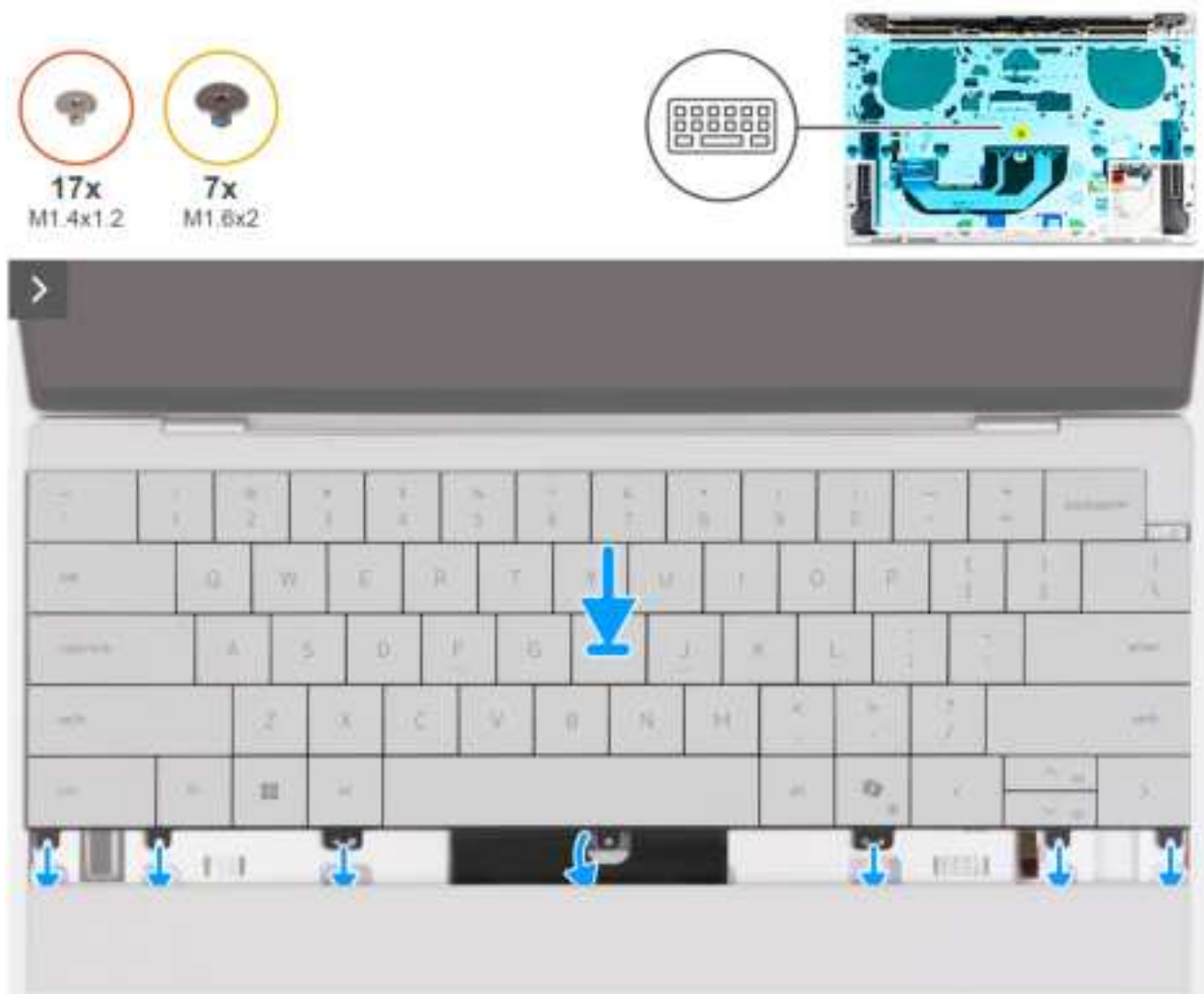
Figure 58. Installing the keyboard
