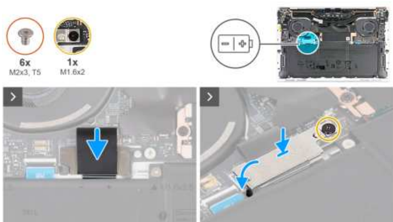
Figure 14. Installing the base cover
