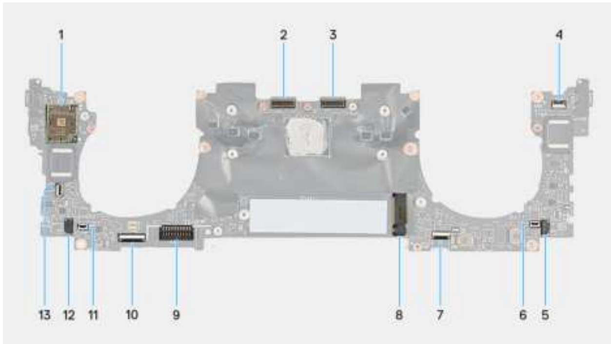
Figure 49. System-board connectors
