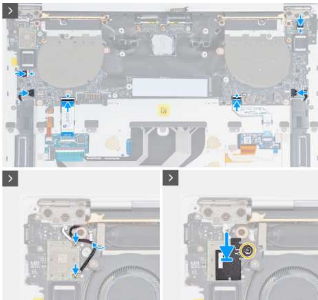
Figure 51. Installing the system board
