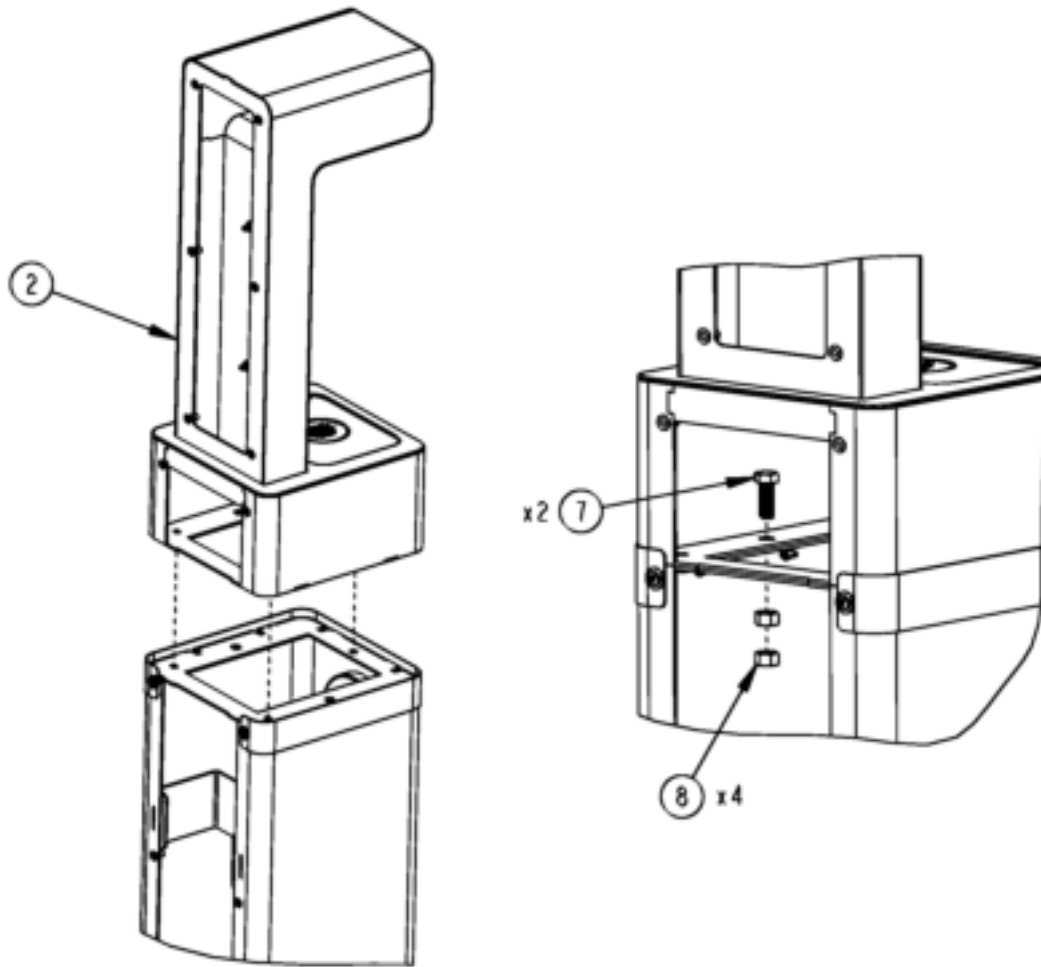
Fig.6 – Alcove assembly
