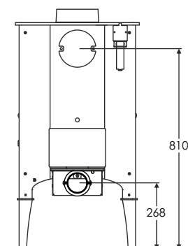
Rear
