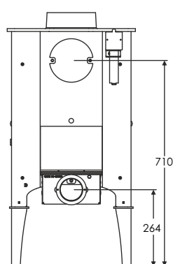
Rear
