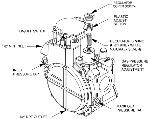
Fig. 12 – Single-Stage Gas Valve
