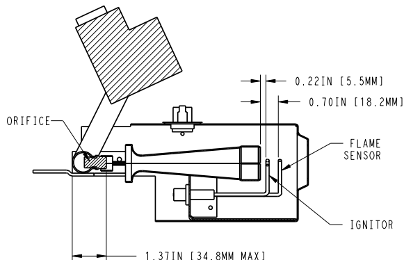
Fig. 13 – Single-Stage Igniter, Flame Sensor, Orifice/Main Burner Relationship
