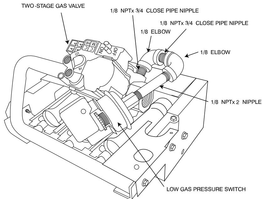
Fig. 9 – Burner Bracket
