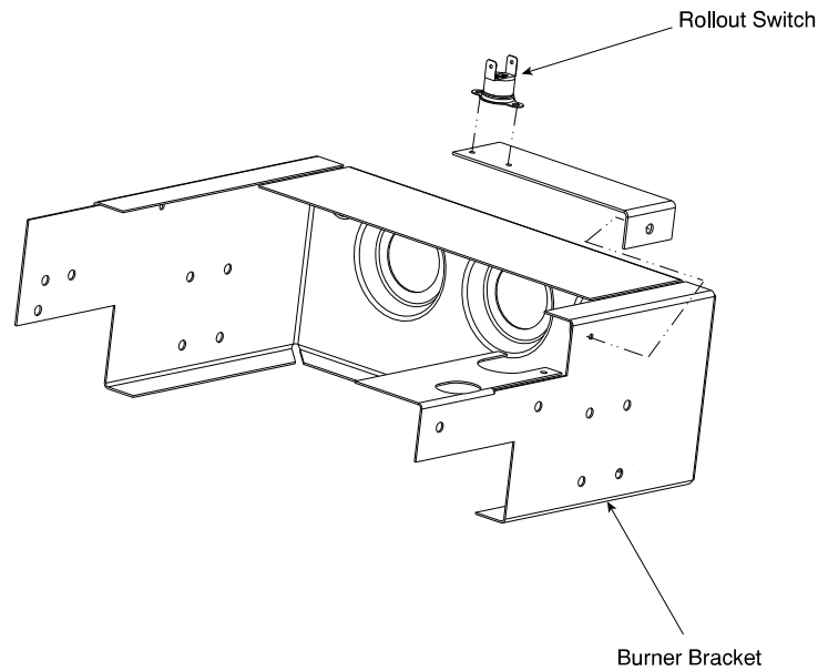
Fig. 9 – Burner Bracket
