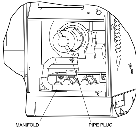
Fig. 4 – Two-Stage Burner Assembly
