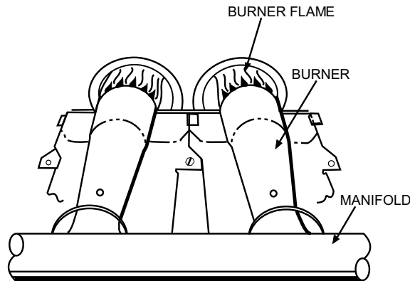
Fig. 6 – Monoport Burner
