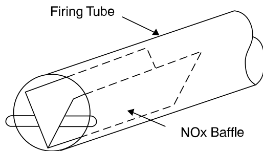
Fig. 1 – Low NOx Baffle Location (California Installations Only) A221556
