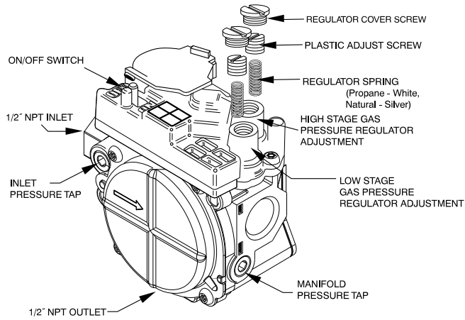
Fig. 2 – Two-Stage Gas Valve
