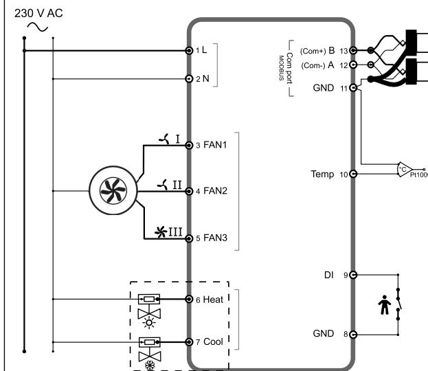
Figure 1 4-pipe wiring
