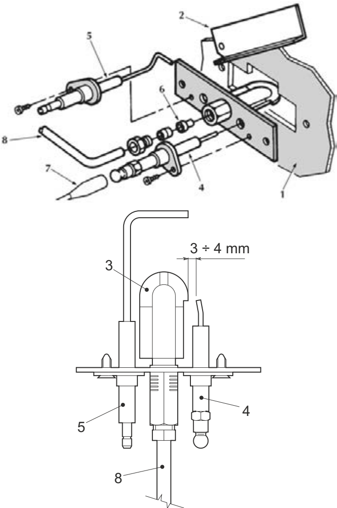
fig. 21 - Pilot burner
