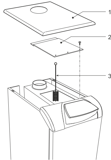
fig. 19 - Boiler cleaning
