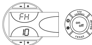
fig. 3 - Boiler lighting
