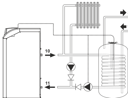
fig. 14 - Diagram of connection to external hot water tank
