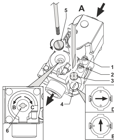
fig. 17 - Pressure adjustment
