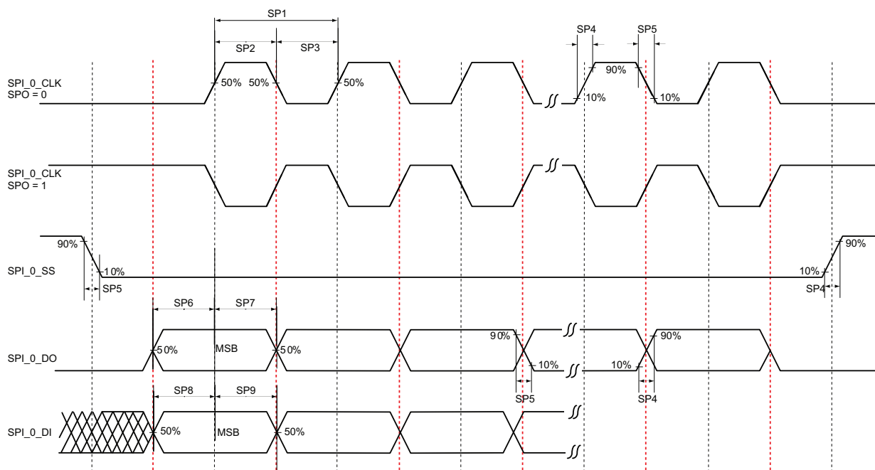
FIGURE 7-7: SPI TIMING FOR A SINGLE FRAME TRANSFER IN MOTOROLA MODE (SPH = 1)
