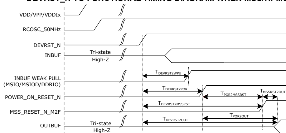
FIGURE 7-3: DEVIRST_N TO FUNCTIONAL TIMING DIAGRAM WHEN MSS/HPMS IS USED
