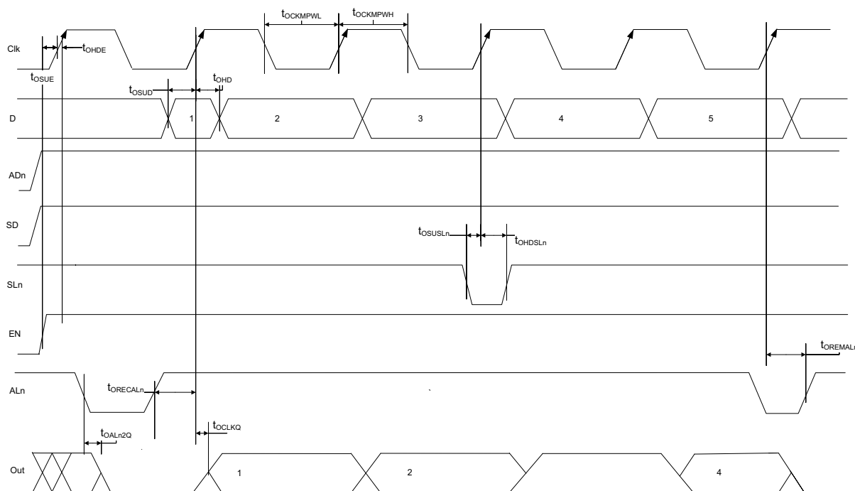
FIGURE 5-7: I/O REGISTER OUTPUT TIMING DIAGRAM
