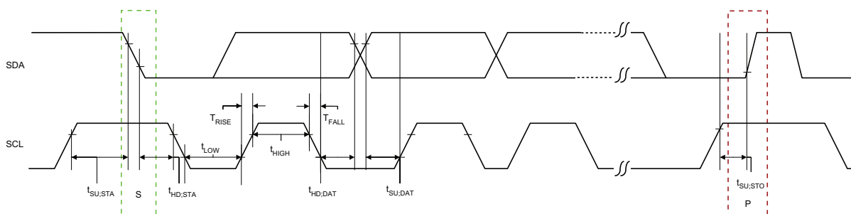
FIGURE 7-5: I 2 C TIMING PARAMETER DEFINITION
