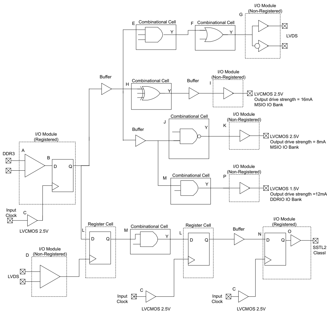
FIGURE 4-1: TIMING MODEL
