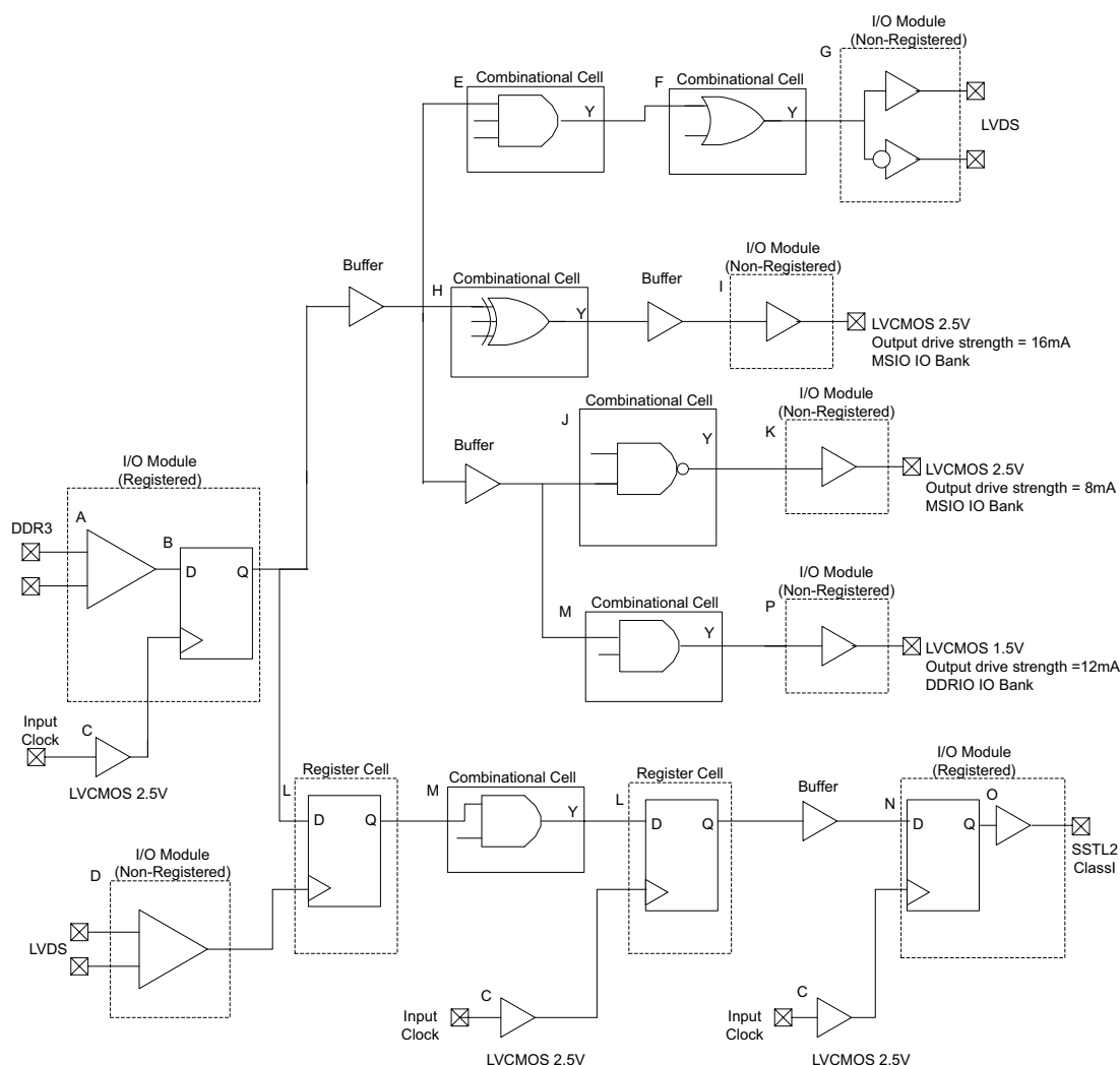
FIGURE 4-1: TIMING MODEL
