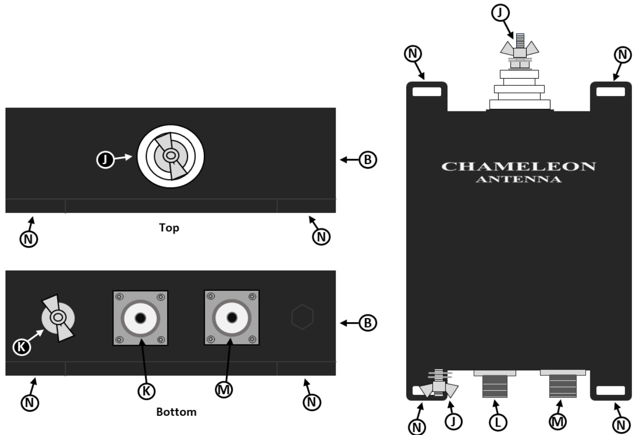
Figure 2. Tuner Unit.
