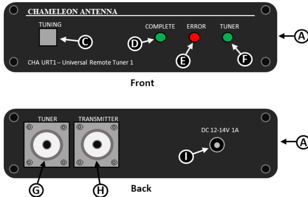
Figure 1. Coupler Unit.
