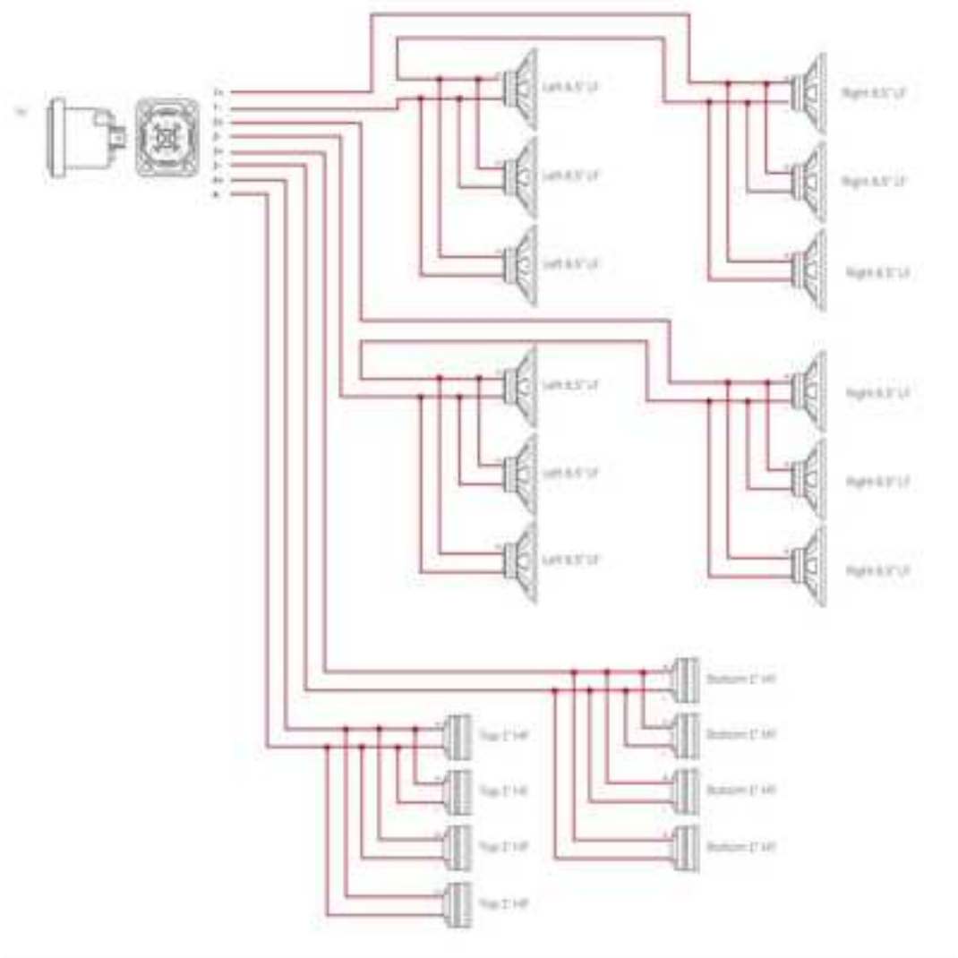
Figure 4.2: Wiring diagram
