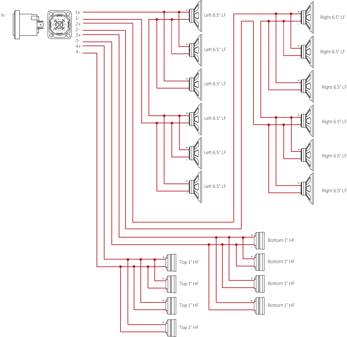
Figure 4.1: Wiring diagram
