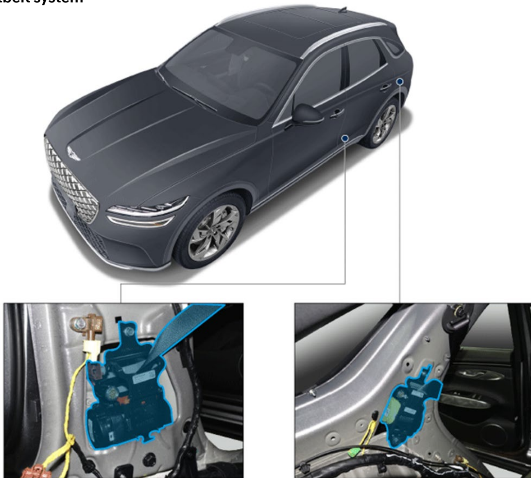
1) Front Seatbelt Pretensioner
