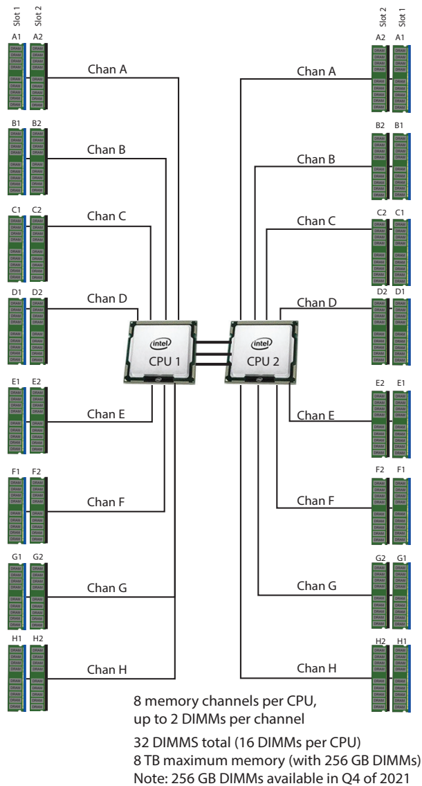
Figure 6 C220 M6 SFF Memory Organization
