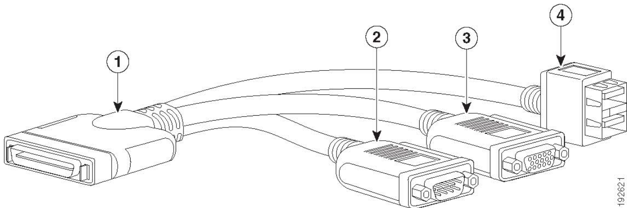
Figure 14 KVM Cable
