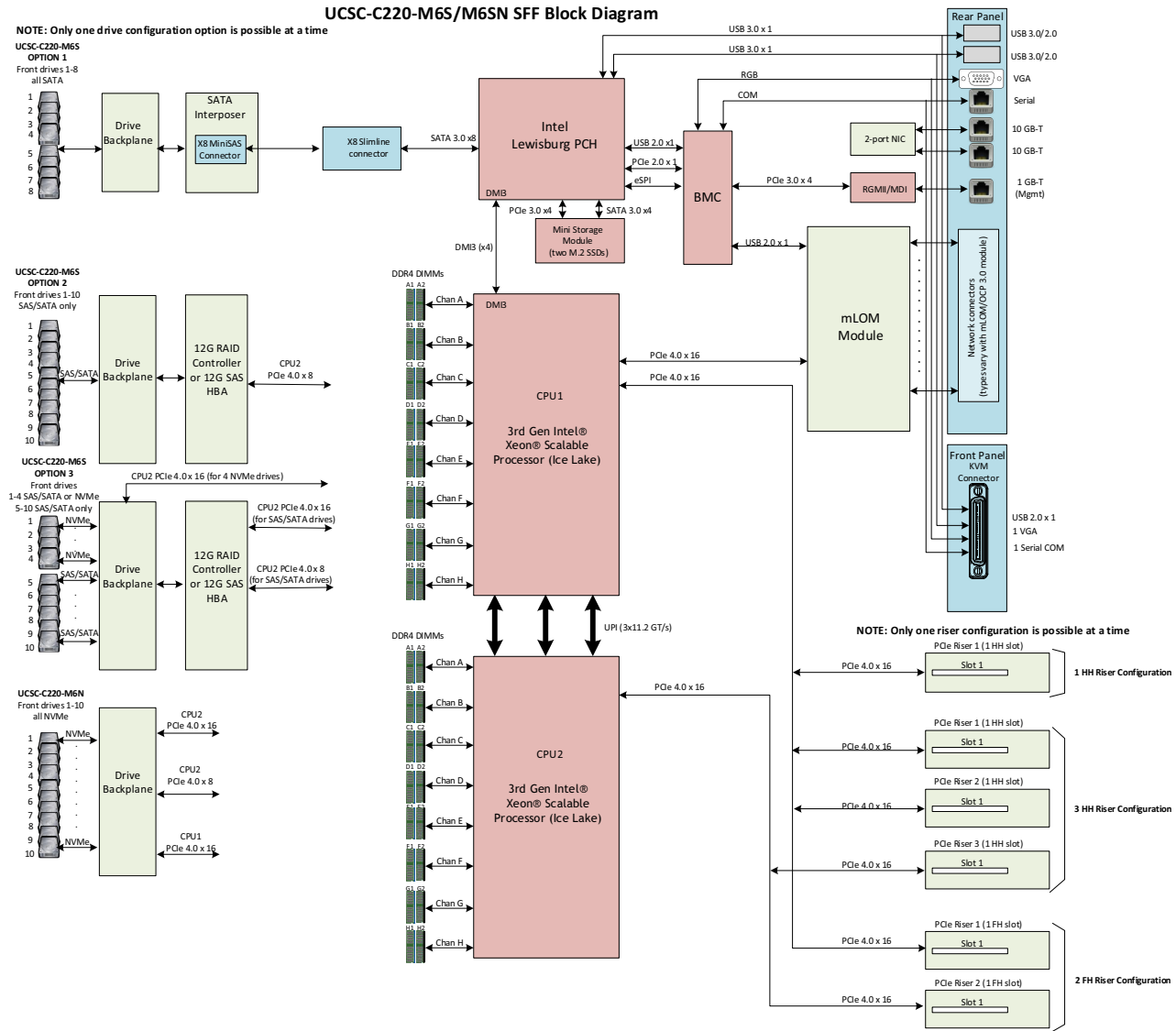
Figure 12 UCSC-C220-M6S/M6N Block Diagram
