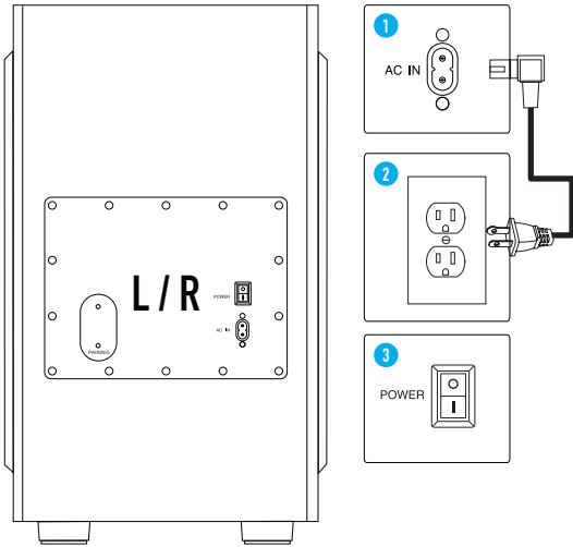
Dual-Opposing 8" Subwoofer
