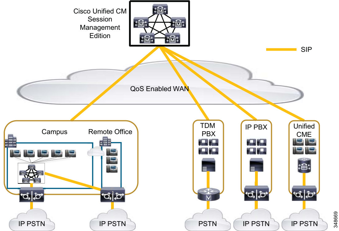
Figure 6-31 Distributed SIP Trunk Model
