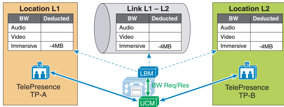
Figure 13-12 Call Flow for End-to-End TelePresence Immersive Video
