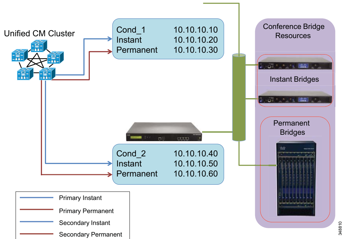
Figure 11-16 Conferencing Redundancy with Unified CM Call Control
