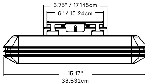
SFC Surface/indirect mount end view
