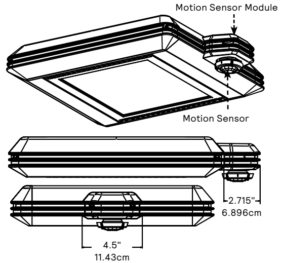
SFC Surface/indirect mount end view
