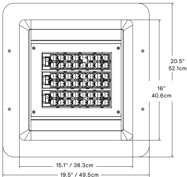
SFCR Recessed mount bottom view
