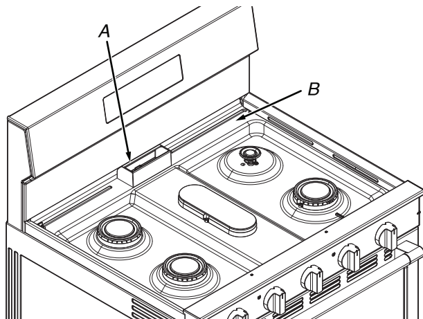
A. Center oven vent cover B. Locating features
