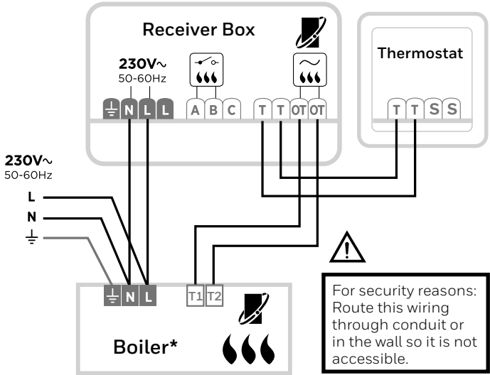
C) OpenTherm boiler
