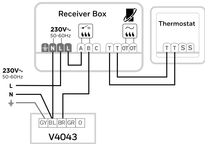
D) Two-port zone valve or S-plan
