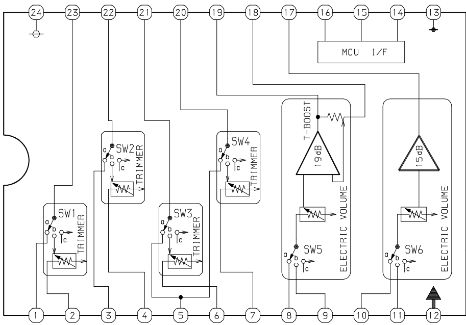
IC, M62491FP
