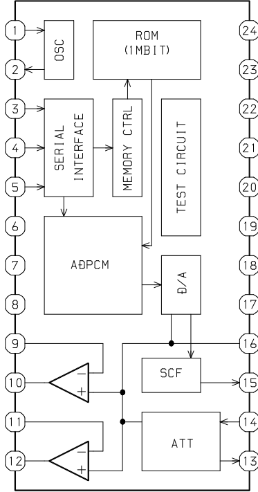
IC, BU9990-03FS
