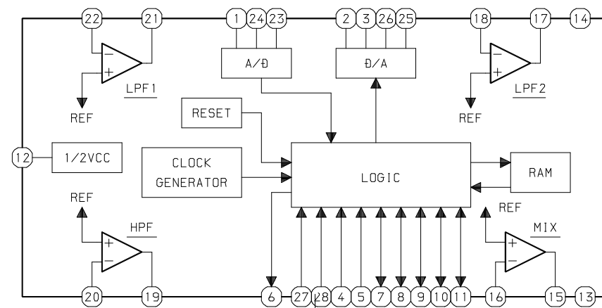
IC, M65847AFP
