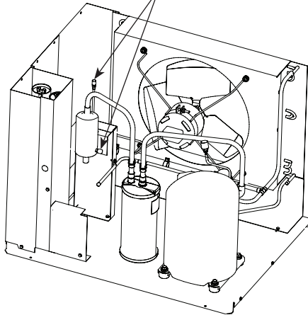
ALTERNATE CONNECTIONS AT CONDENSING UNIT SCHRAEDER VALVES
