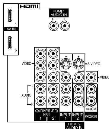
Rear Panel
