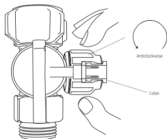
Figure 3 - SmartTee™ Quick Connect Fitting
