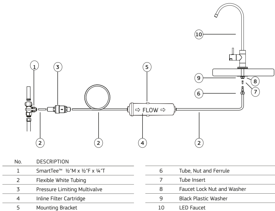
Figure 1 - System Diagram
