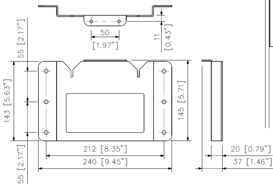
Wall bracket
