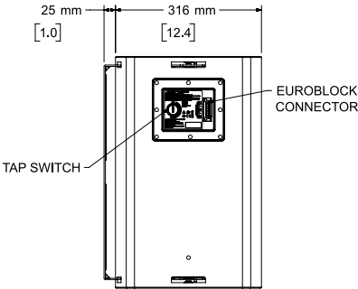
Rear View BRACKET SHOWN IN SIDE LOCATION
