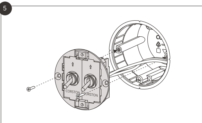
Screw the chassis into the back box.
