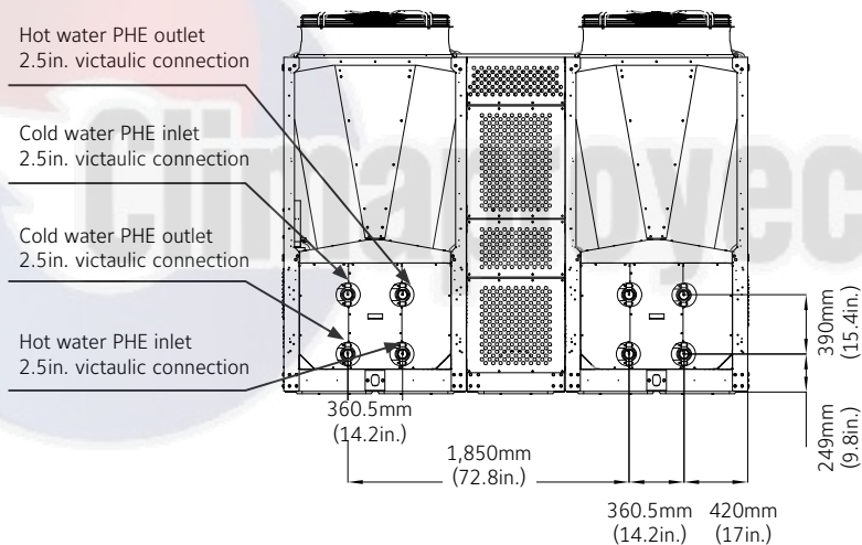
Control panel side (YMAE two-pipe / four-pipe unit)
