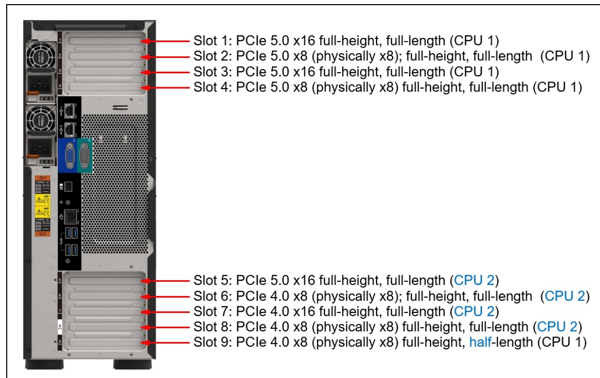
Figure 8. ST650 V3 PCIe slots
