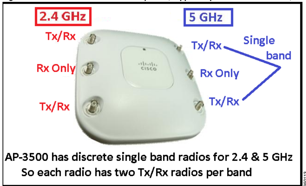
Figure 54 AP 3500i/e is a 2x3:2 System (Supports up to 2 Transmit Chains)
