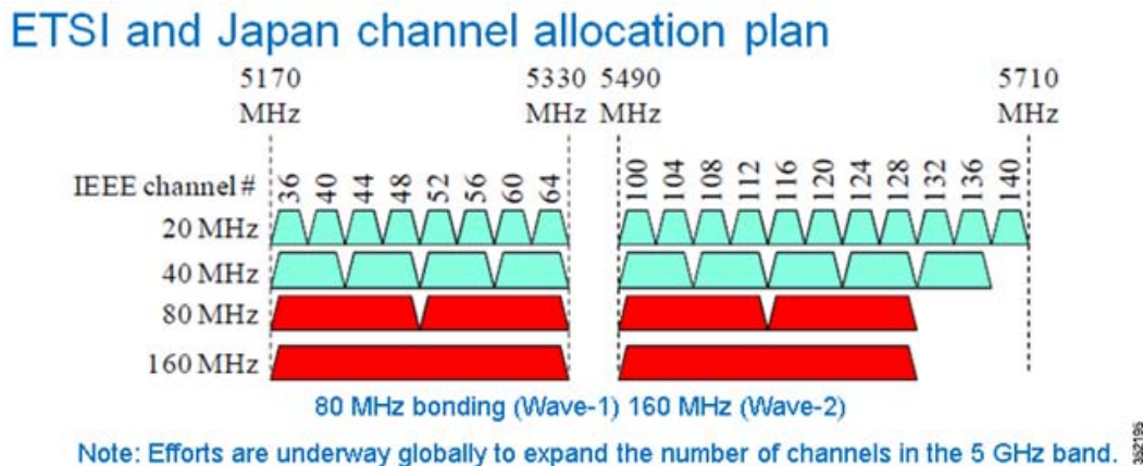
Figure 83 Current Channel Allocation Plan - ETSI Theater
