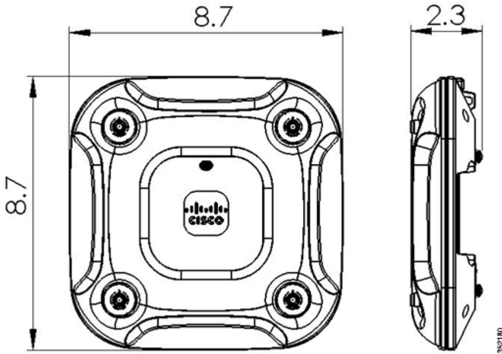
Figure 10 3700 Mechanical Drawing
