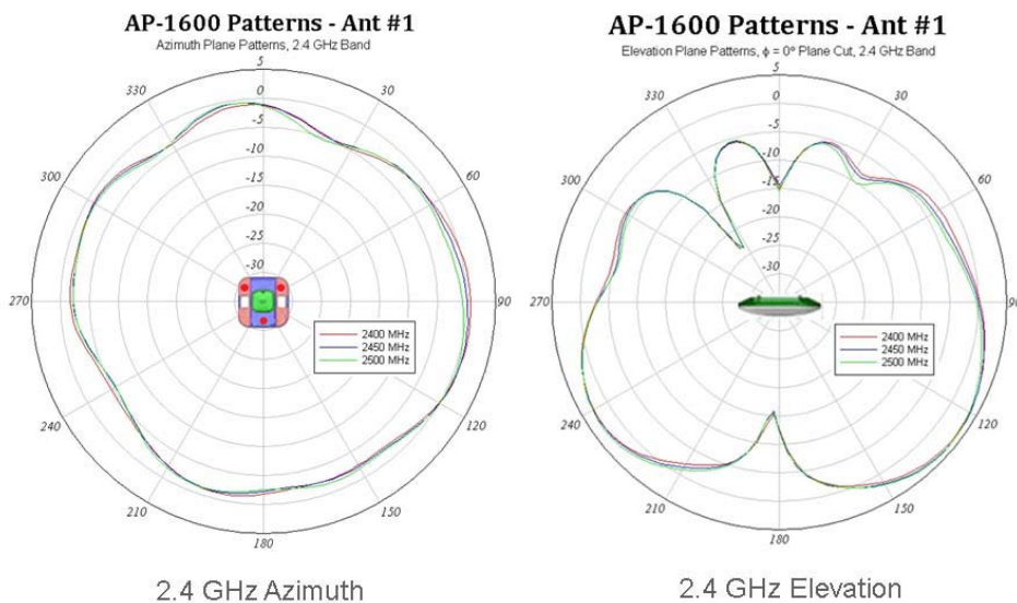
Figure 47 Radiation Patterns for the AP 1600i @ 2.4 GHz AP-1600 2.4 GHz antenna patterns
