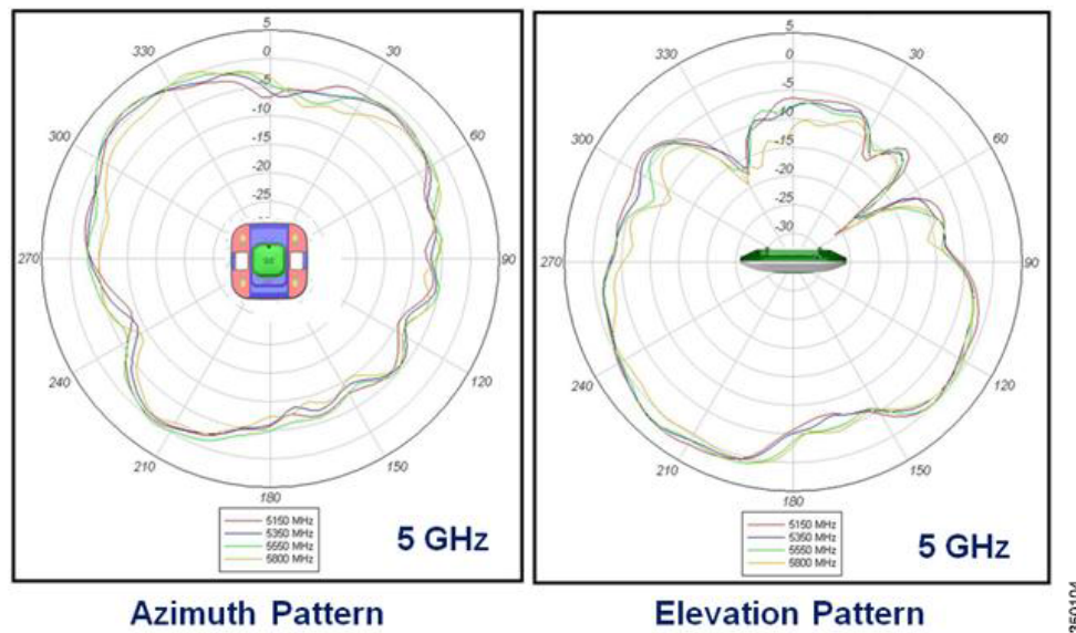
Figure 44 Radiation Patterns for the AP 3600i @ 5 GHz
