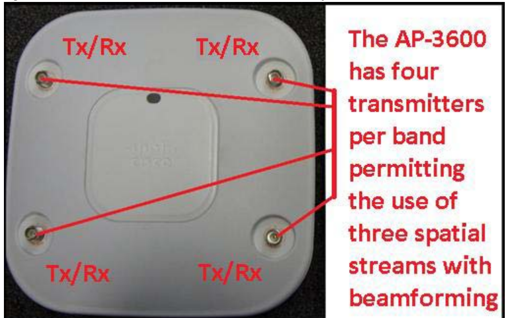
Figure 56 AP 3600: 4 Transmitters and 4 Receivers per Radio Band
