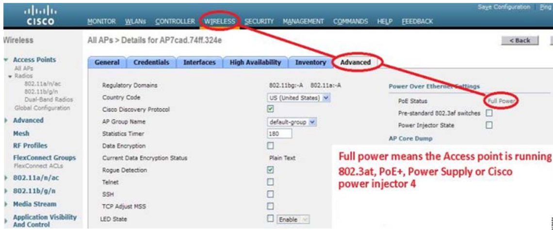
Figure 80 AP 3700 Running in Full Power Mode when it has 18 Watts or More of Available Power
