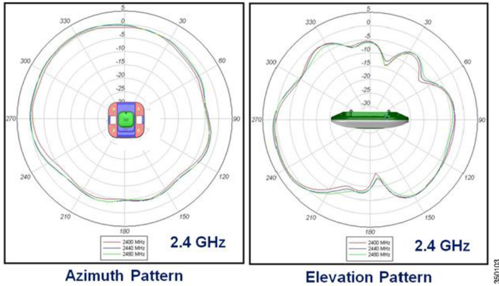
Figure 43 Radiation Patterns for the AP 3600i @ 2.4 GHz
