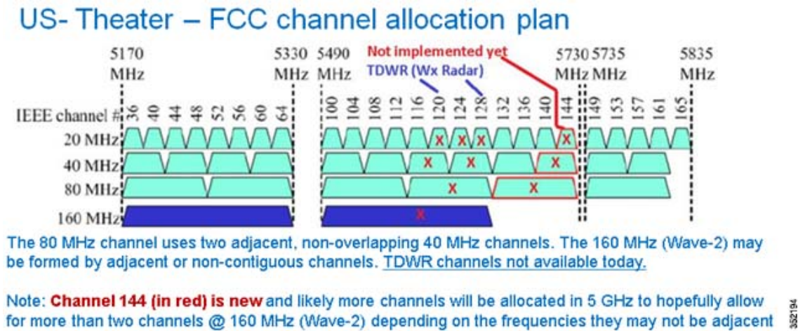
Figure 82 Current Channel Allocation Plan - US Theater
