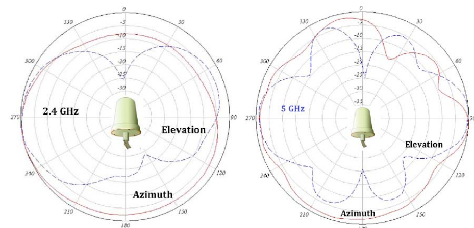
Figure 37 Radiation Patterns for the AIR-ANT2544V4M-R Dual-Band Omni Antenna
