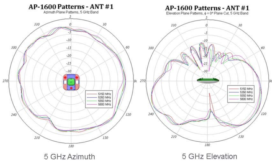
Figure 48 Radiation Patterns for the AP 1600i @ 5 GHz AP-1600 5 GHz antenna patterns
