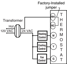
HEAT/COOL 4-WIRE SINGLE TRANSFORMER
