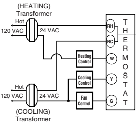
HEAT/COOL 5-WIRE TWO TRANSFORMER
