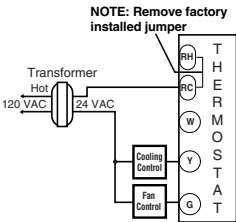
COOL ONLY 3-WIRE SINGLE TRANSFORMER
