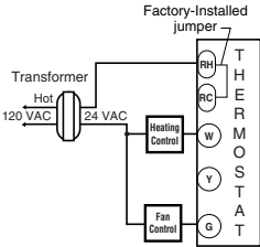
HEAT ONLY 3-WIRE SINGLE TRANSFORMER
