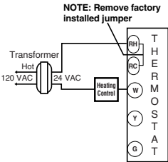
HEAT ONLY 2-WIRE SINGLE TRANSFORMER
