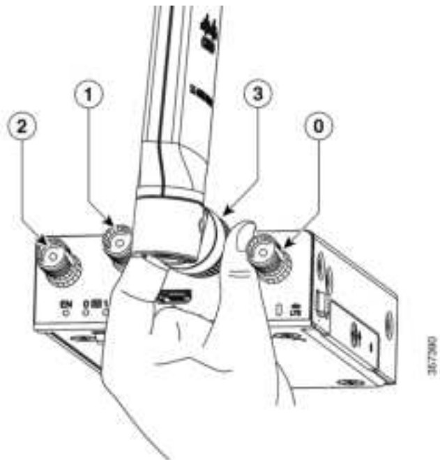
Figure 4: Attaching the Antennas
