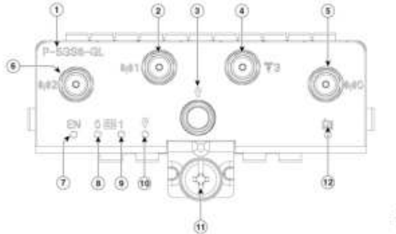
Figure 3: 5G Pluggable Interface Module - P-5GS6-GL
