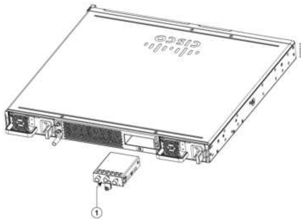
Figure 1: Pluggable Interface Module in a Cisco 8300-1N1S-4T2X/6T
