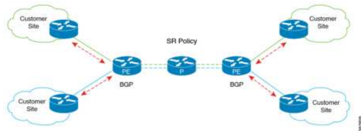
Figure 1: EVPN VPWS over SR-TE Architecture
