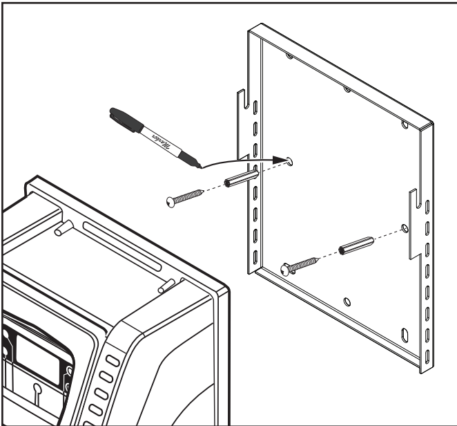
Figure 5. Controller Mount
