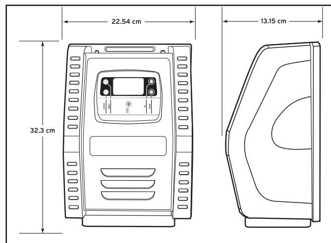
Figure 1. Controller Dimensions
