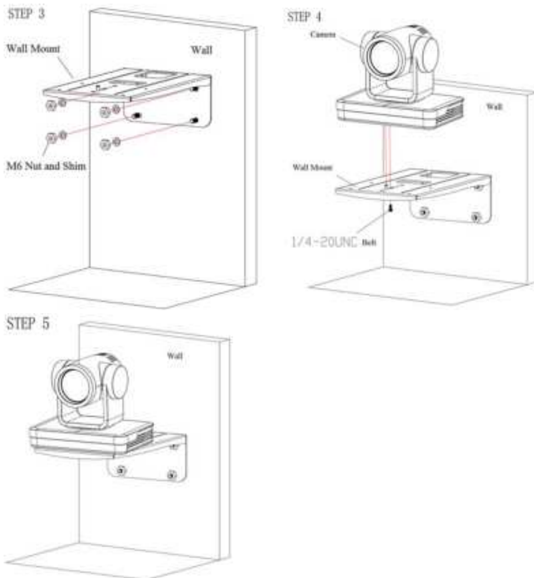
Figure1-3 Steps of Wall Mount
