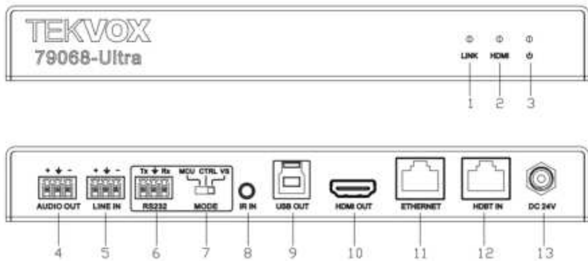
Figure1-2 Receiver Hardware
