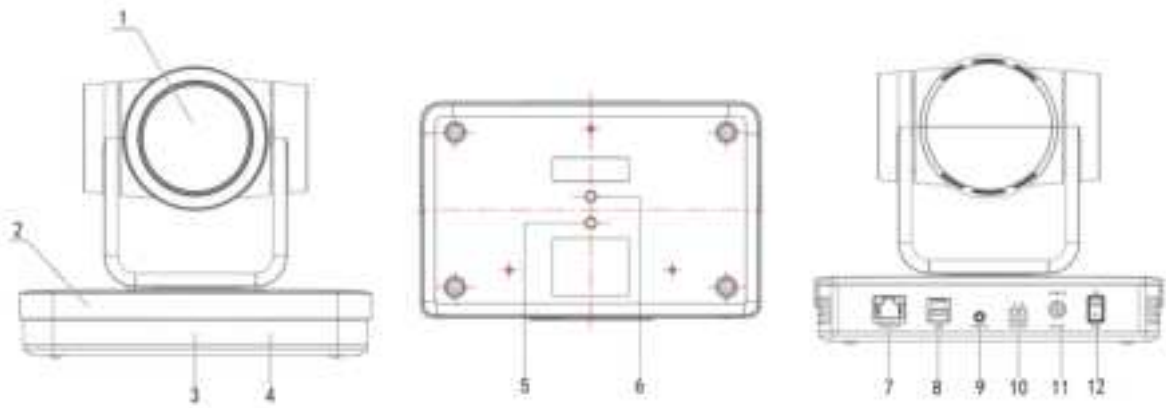
Figure1-1 Camera Hardware
