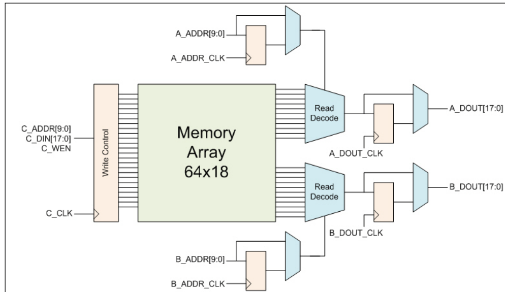
Figure 69 • Simplified Block Diagram of RAM64x18
