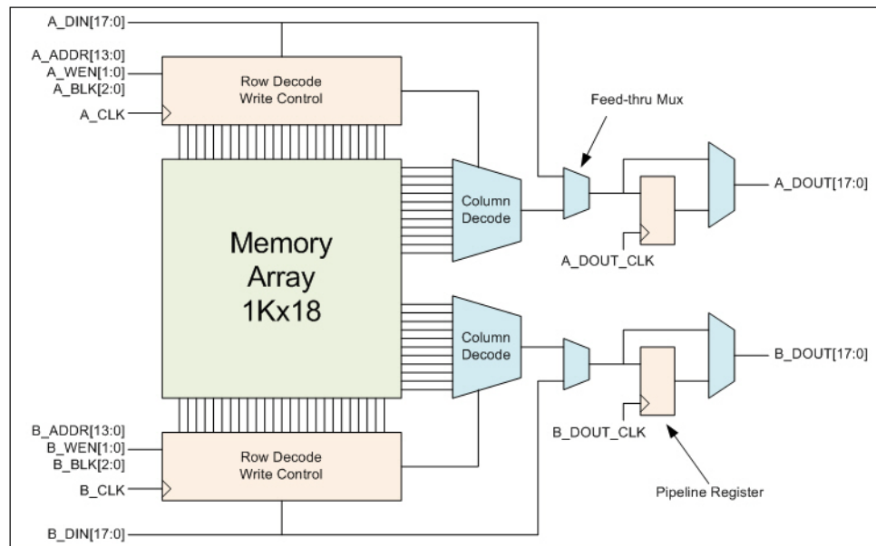
Figure 68 • Simplified Block Diagram of RAM1K18
