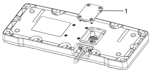
1 Cable Cover with M3 Screws (4)
