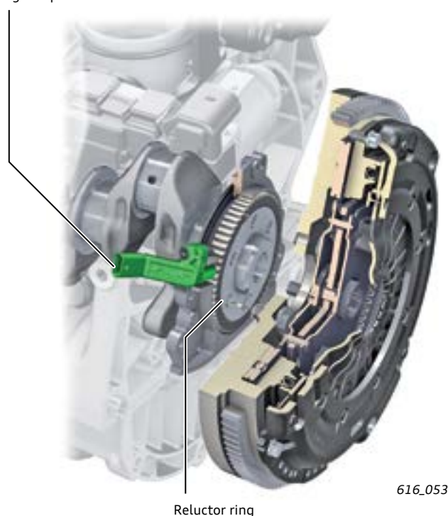
Engine Speed Sensor G28
