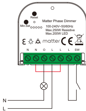
Method 2: Without neutral
