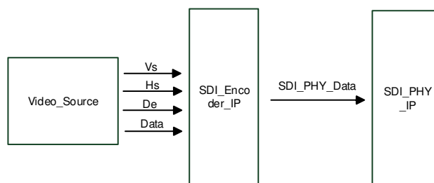
Figure 3-2 Gowin SDI Encoder IP Block Diagram
