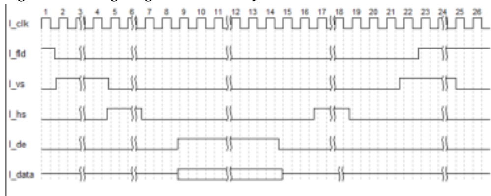
Figure 3-4 Timing Diagram of Video Input Interface
