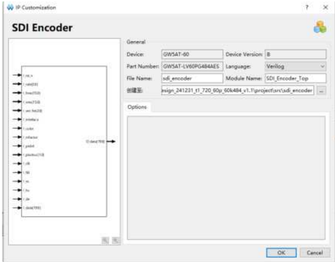
Figure 4-3 Gowin SDI Encoder IP Configuration Interface
