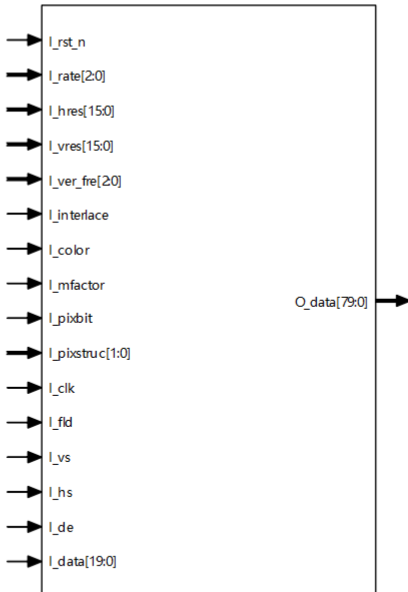
Figure 3-3 Gowin SDI Encoder IP Port Diagram
