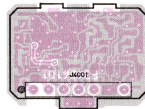
J4001 To 144-Mother Unit (See Page 4B-3) 1. SHIFT 2. VCV 3. MOD 4. SAVED 5. PLL OUT 6. GND 7. OUT obverse view of connector side
