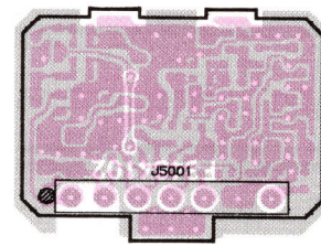
J5001 To 430-Mother Unit (See Page 4C-3) 1. SHIFT 2. VCV 3. MOD 4. SAVE3 5. PLL OUT 6. GND 7. OUT
