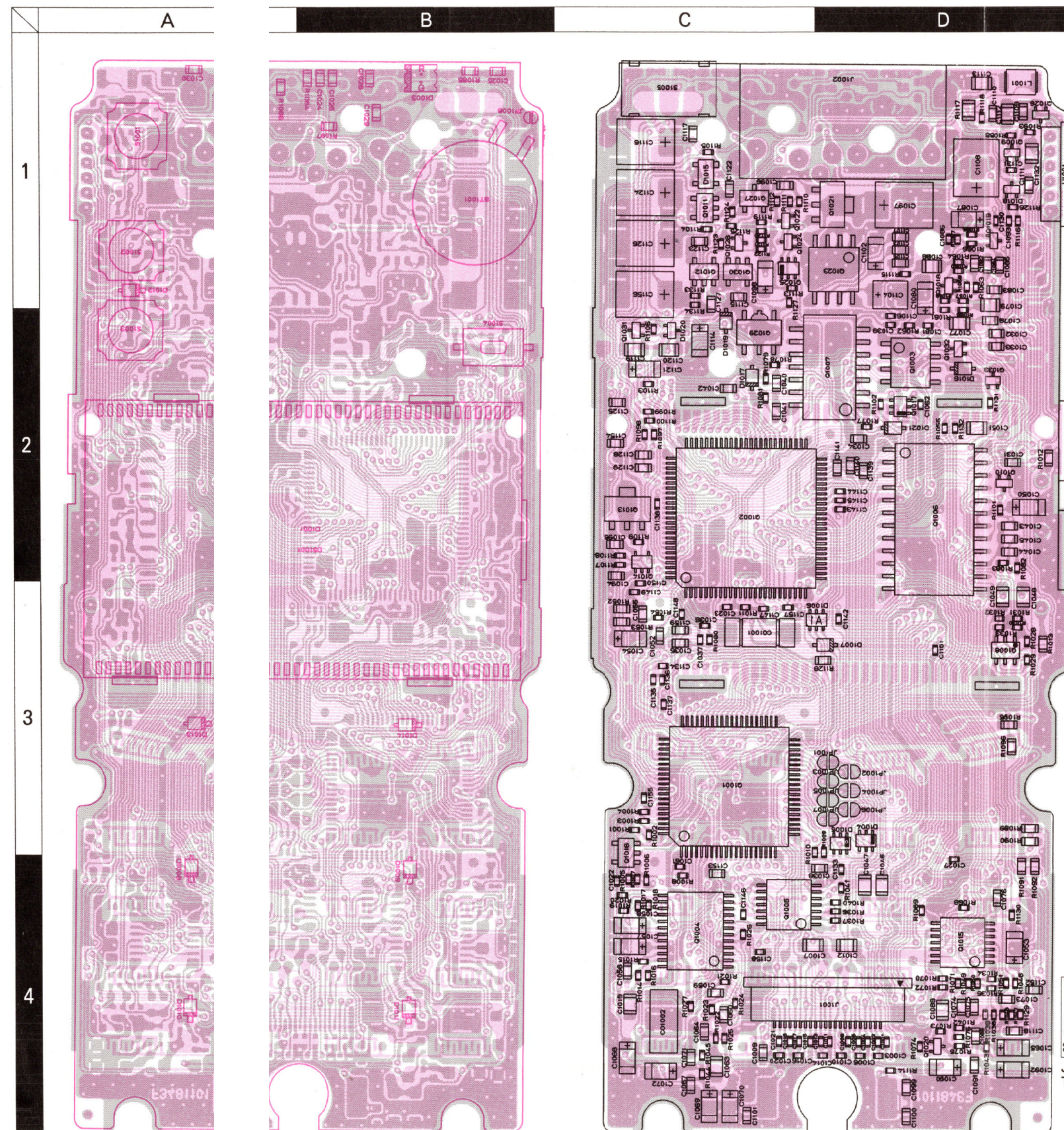
obverse view of component side
