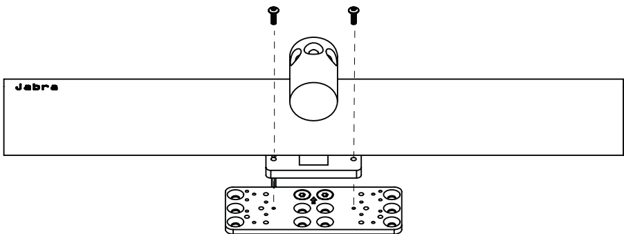
Bottom View
