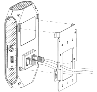
Figure 9 Attaching AP311H to wall mounting plate
