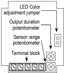
Fig.3 LED Jumper Settings
