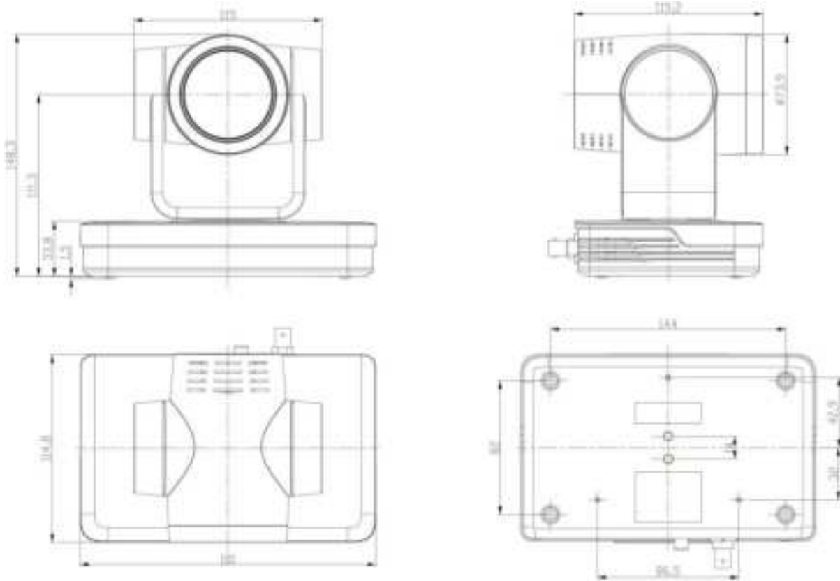
Figure 2.2 Product Dimensions
