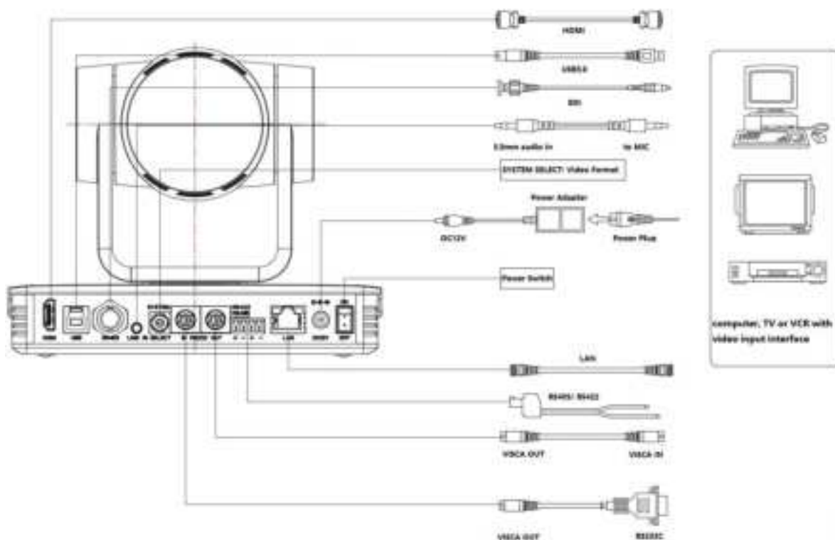
Figure 1.3 Wiring Diagram
