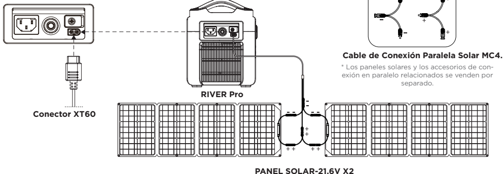
RIVER Pro Charging Port
