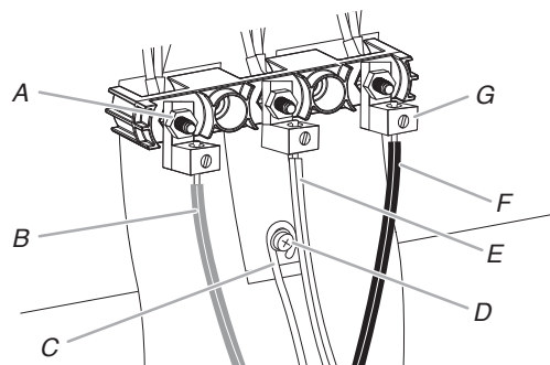
A. 10-32 hex nut B. Line 2 (red) C. Bare (green) ground wire D. Ground-link screw E. Neutral (white) wire F. Line 1 (black) G. Terminal lug
