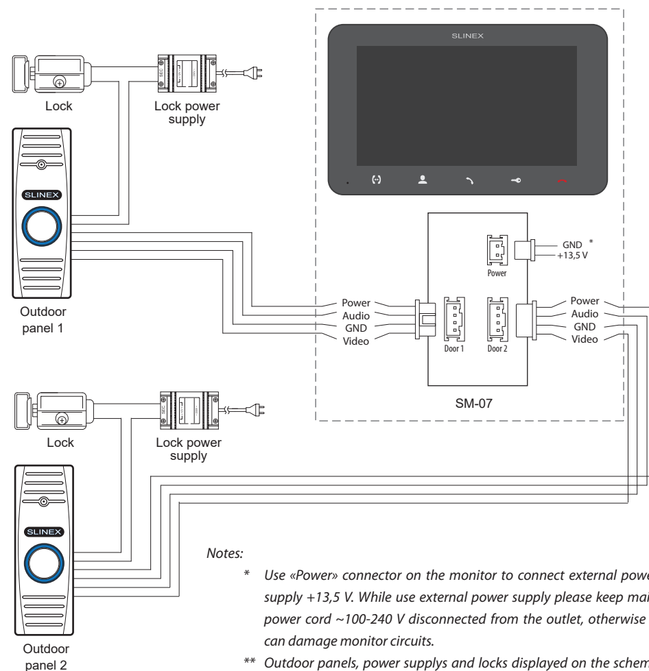
Diagram 1. SM-07 monitor, outdoor panels and locks connection.
