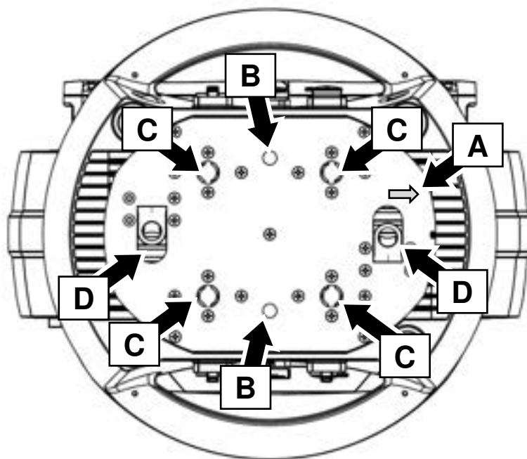
Figure 2. Fixture baseplate
