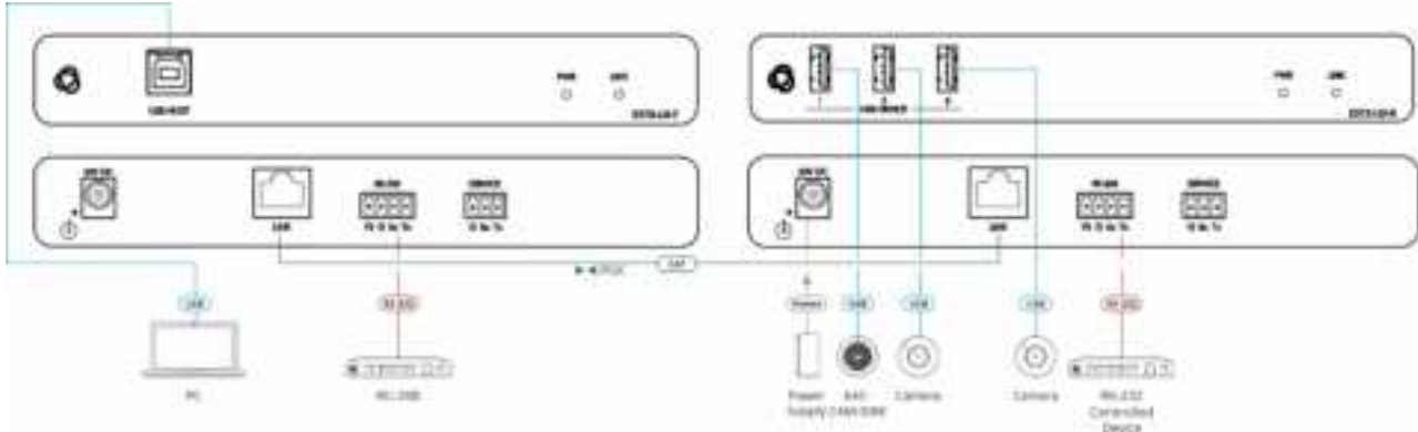
Figure 3: Connecting to the EXT3-U3-T/R
