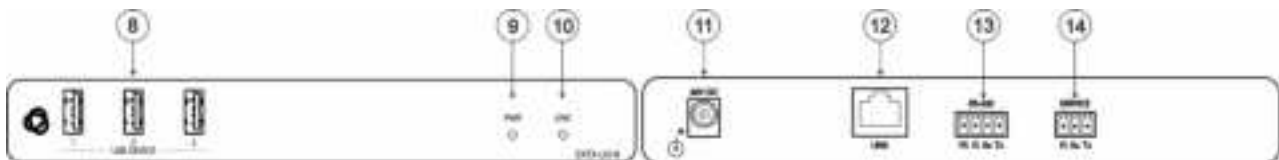
Figure 2: EXT3-U3-R Receiver
